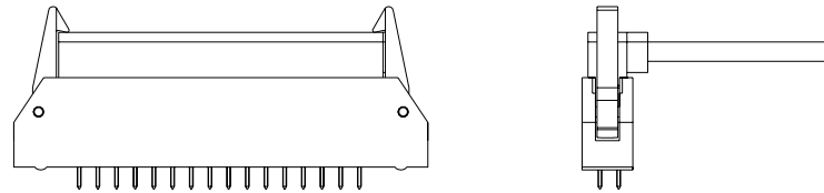
ASSEMBLY SHOWN MATED WITH MERITEC .125 INCH PITCH LATCH AND EJECT HEADER
